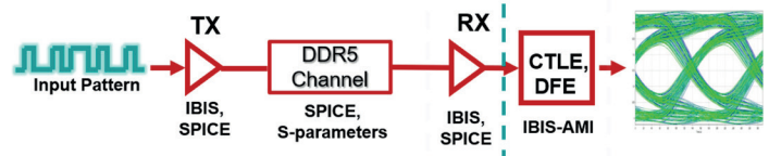
Figure 8(A). Example for DDR interface.
